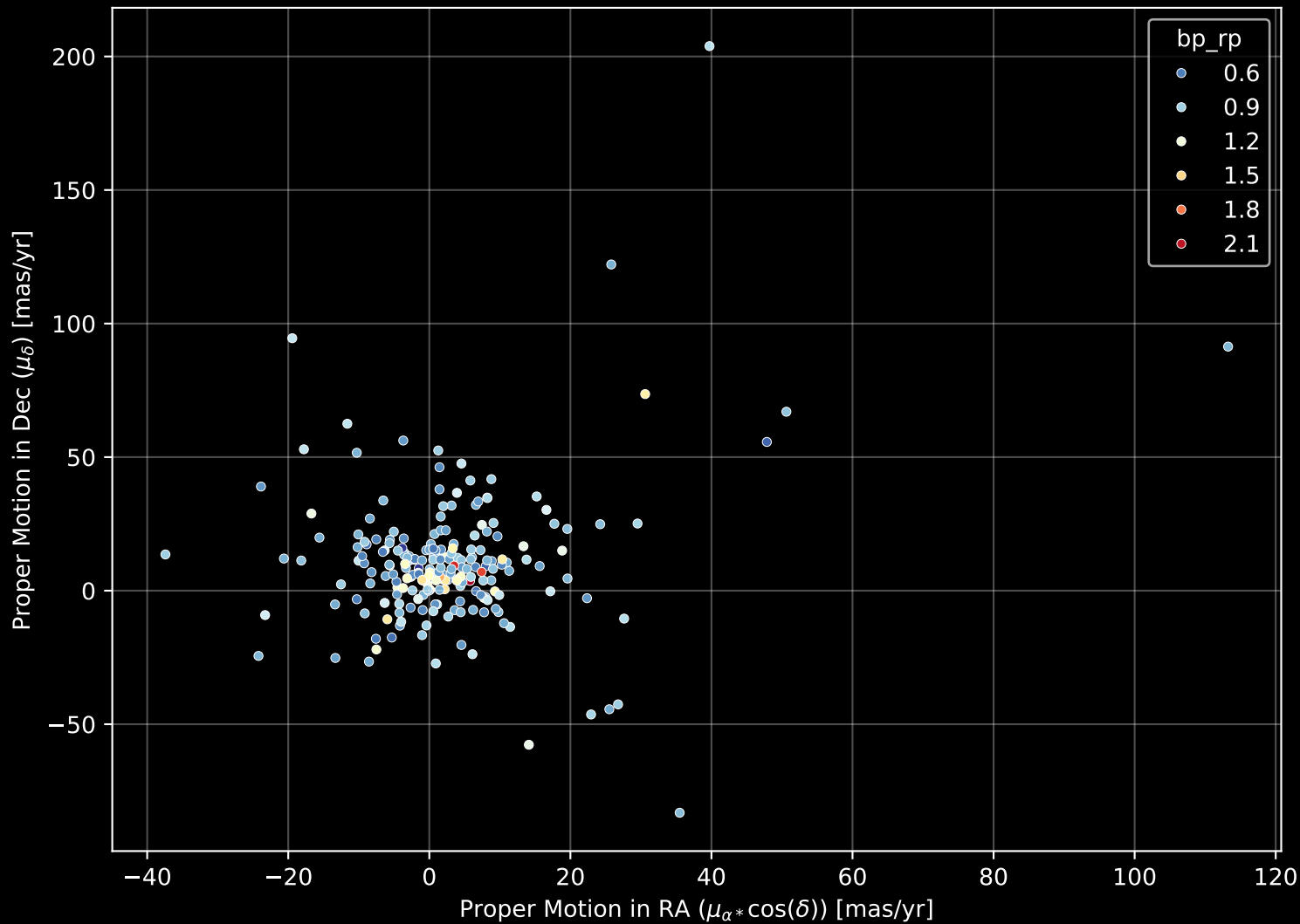
GALAH DR4 Field: [7186] Proper Motion Diagram (n= 218)
