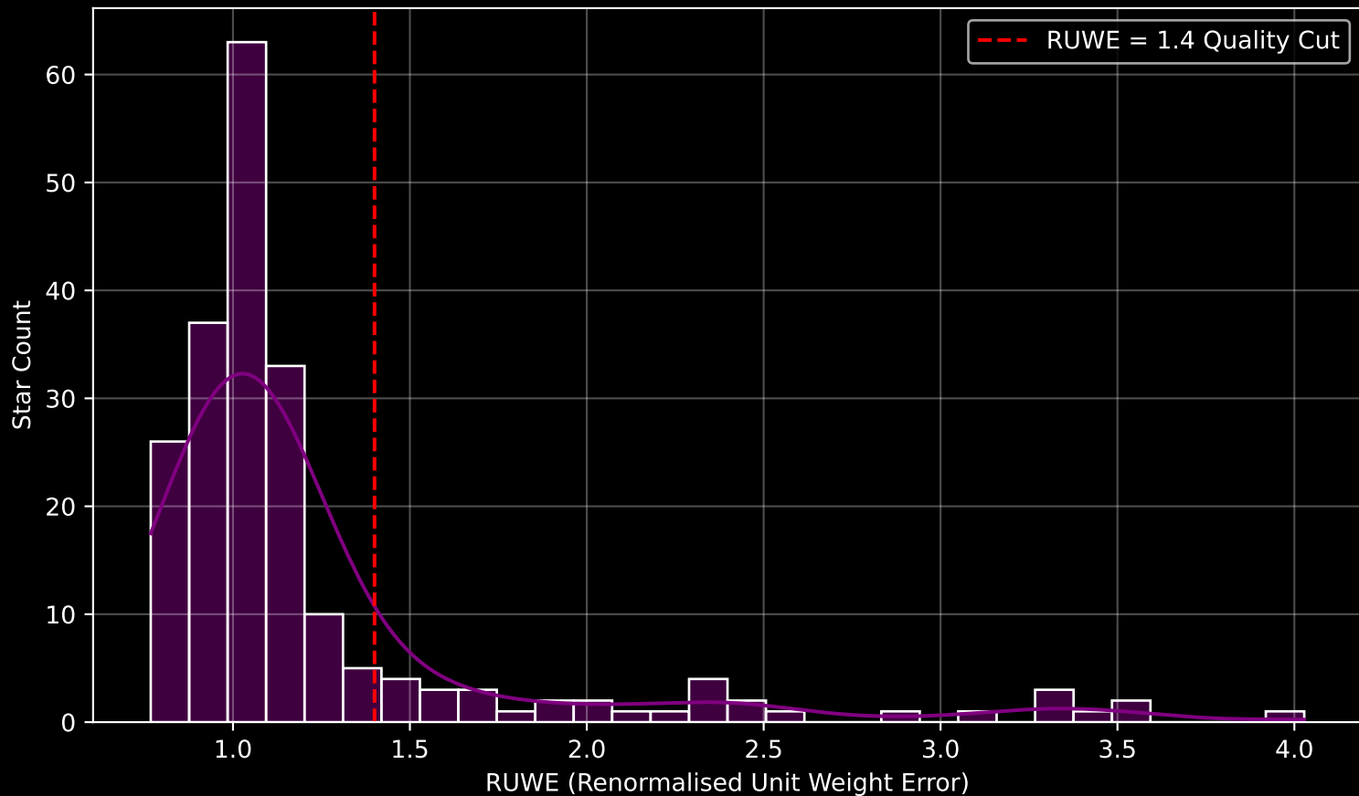
GALAH DR4 Field [7186] RUWE Distribution (n= 207)
