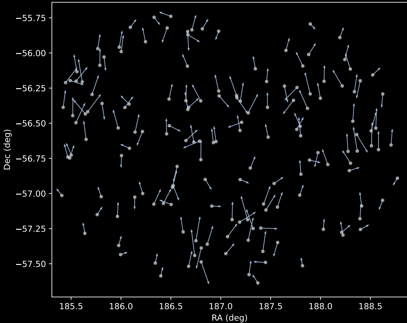
GALAH DR4 Cluster 1 Proper Motion Vectors (n=156)
