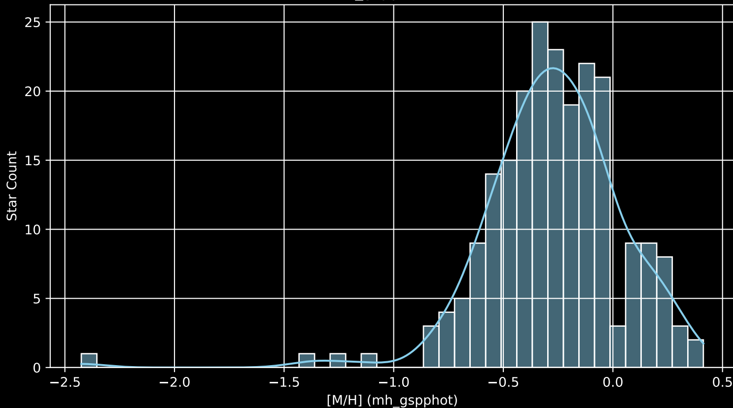
GALAH DR4 Field: [7186] [M/H] (mh_gspphot) (n= 218)
