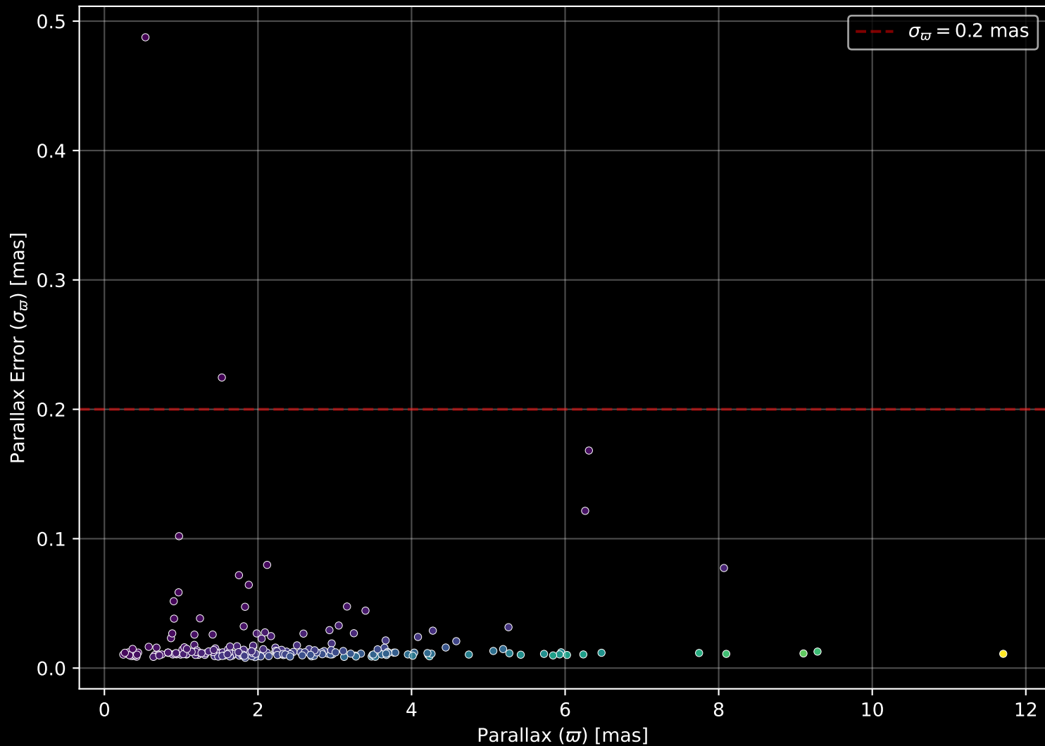
GALAH DR4 Field: [7186] Parallax Quality (n= 218)
