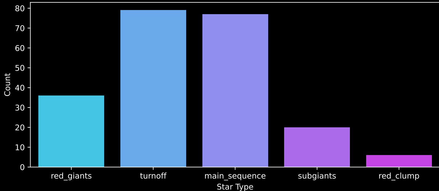
GALAH DR4 Field: [7186] Count plot of Star Type
